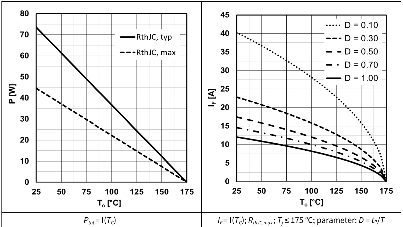
Figure 1 Power dissipation
