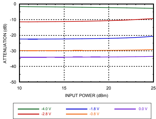
Attenuation vs. Input Power over Vctrl Vctrl1 = Vctrl2
