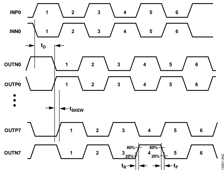
Figure 2. Timing Diagram
