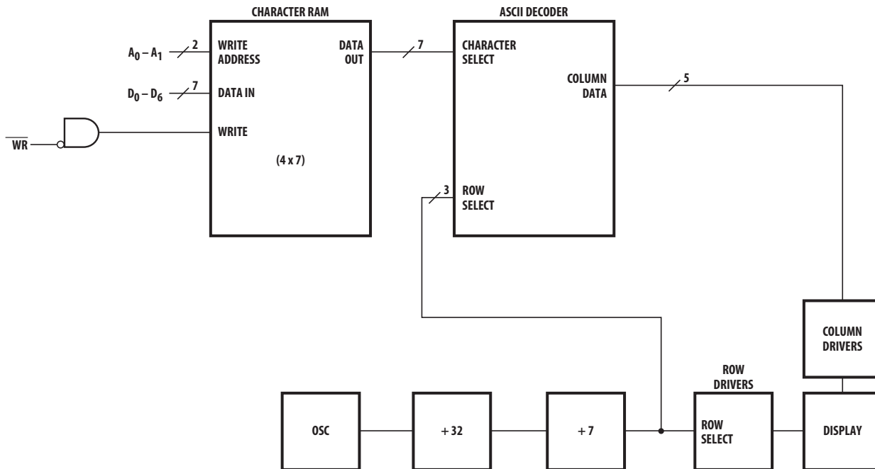
Figure 1: Display Internal Block Diagram
