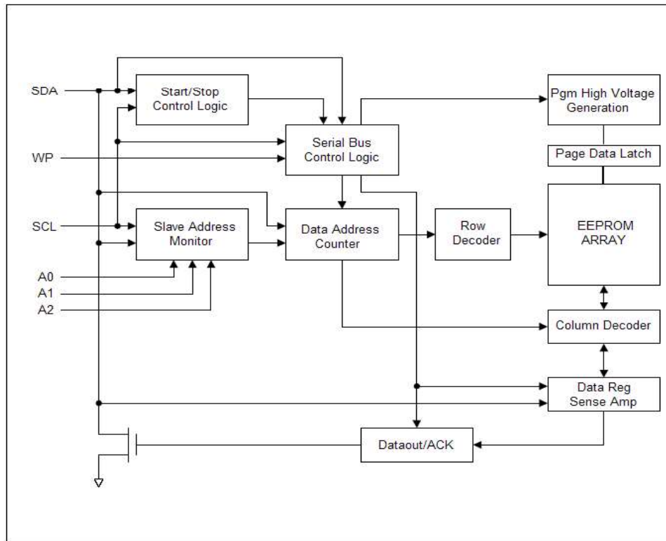
Block Diagram
