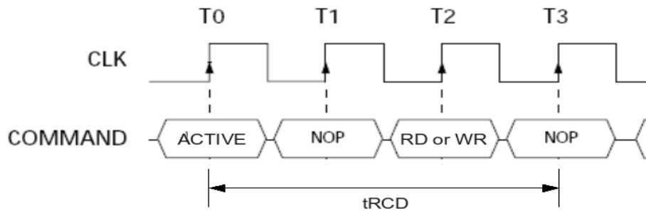
Figure 24. Meeting tRCD (min) When 2 < tRCD \text{ (min)}/tCK \leq 3
