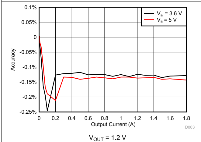
Figure 6-3. DCDC3 Accuracy
