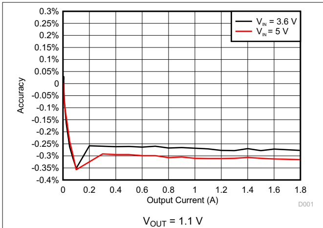
Figure 6-1. DCDC1 Accuracy
