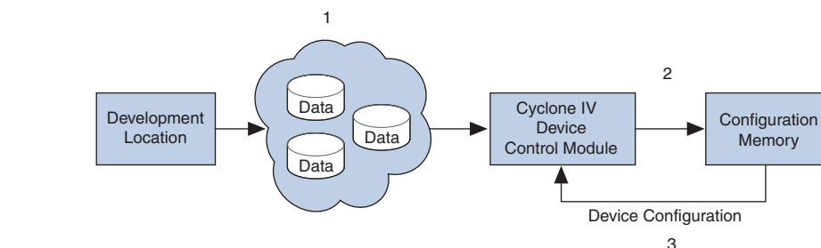
Figure 8-30. Functional Diagram of Cyclone IV Device Remote System Upgrade
