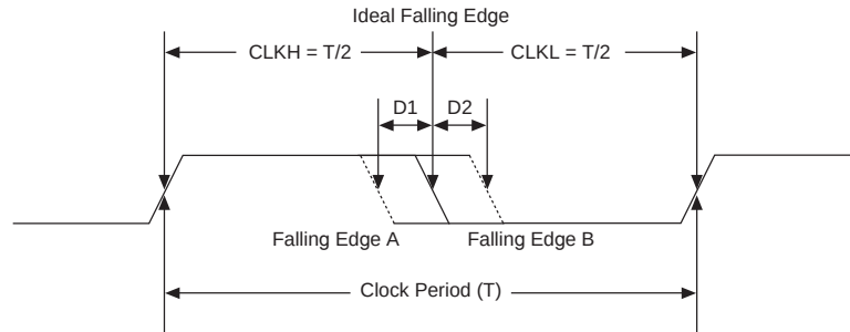
Figure 4–11. Duty Cycle Distortion
