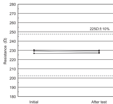
Coil resistance
