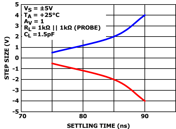
FIGURE 26. STEP SIZE vs SETTILING TIME
