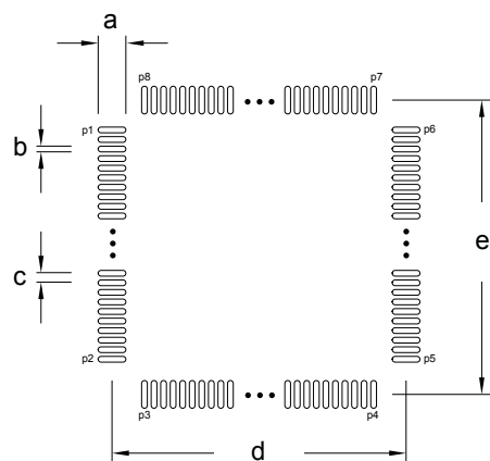
Figure 9.2. TQFP64 PCB Land Pattern
