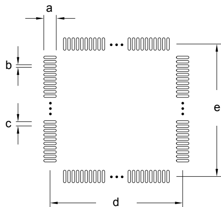
Figure 9.3. TQFP64 PCB Solder Mask
