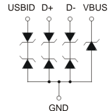
Schematic
