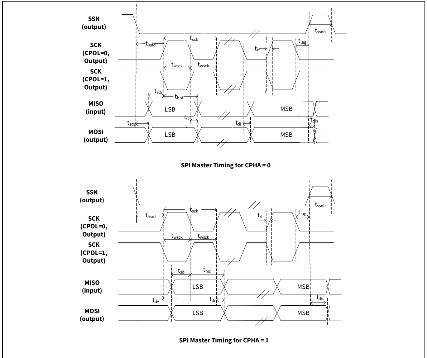
Figure 30 SPI timing
