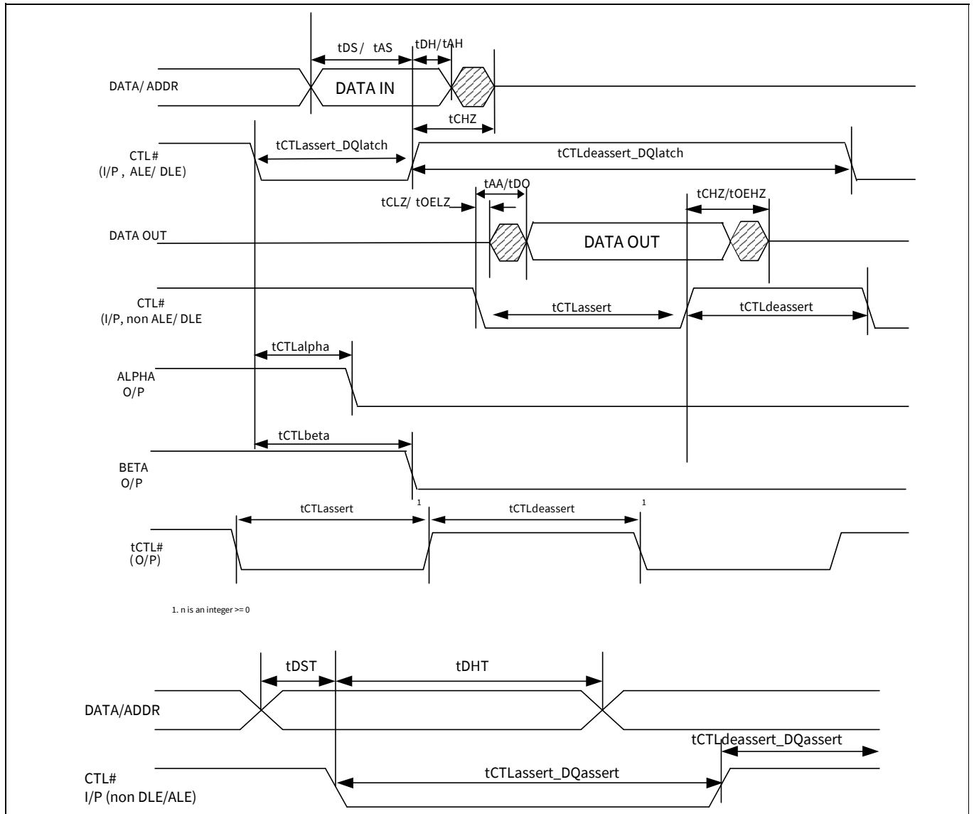
Figure 13 GPIF II timing in asynchronous mode
