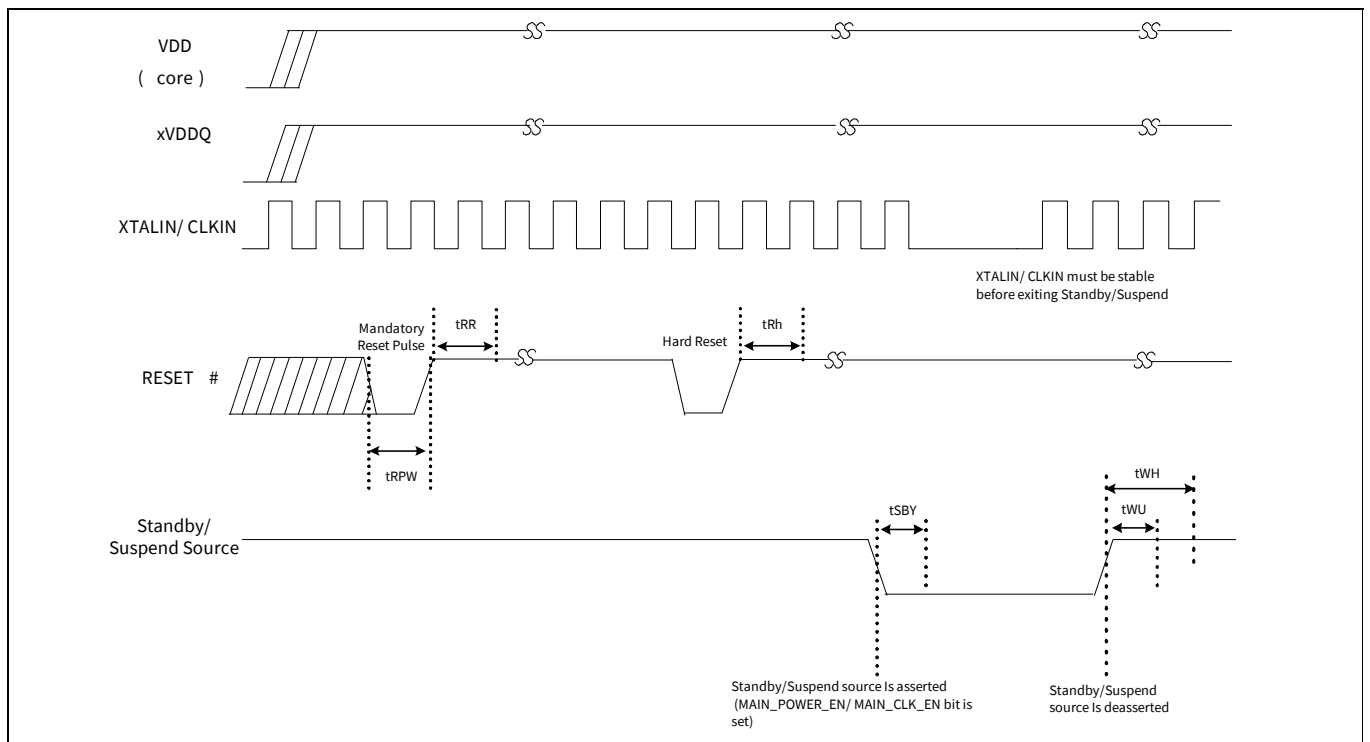
Figure 31 Reset sequence
