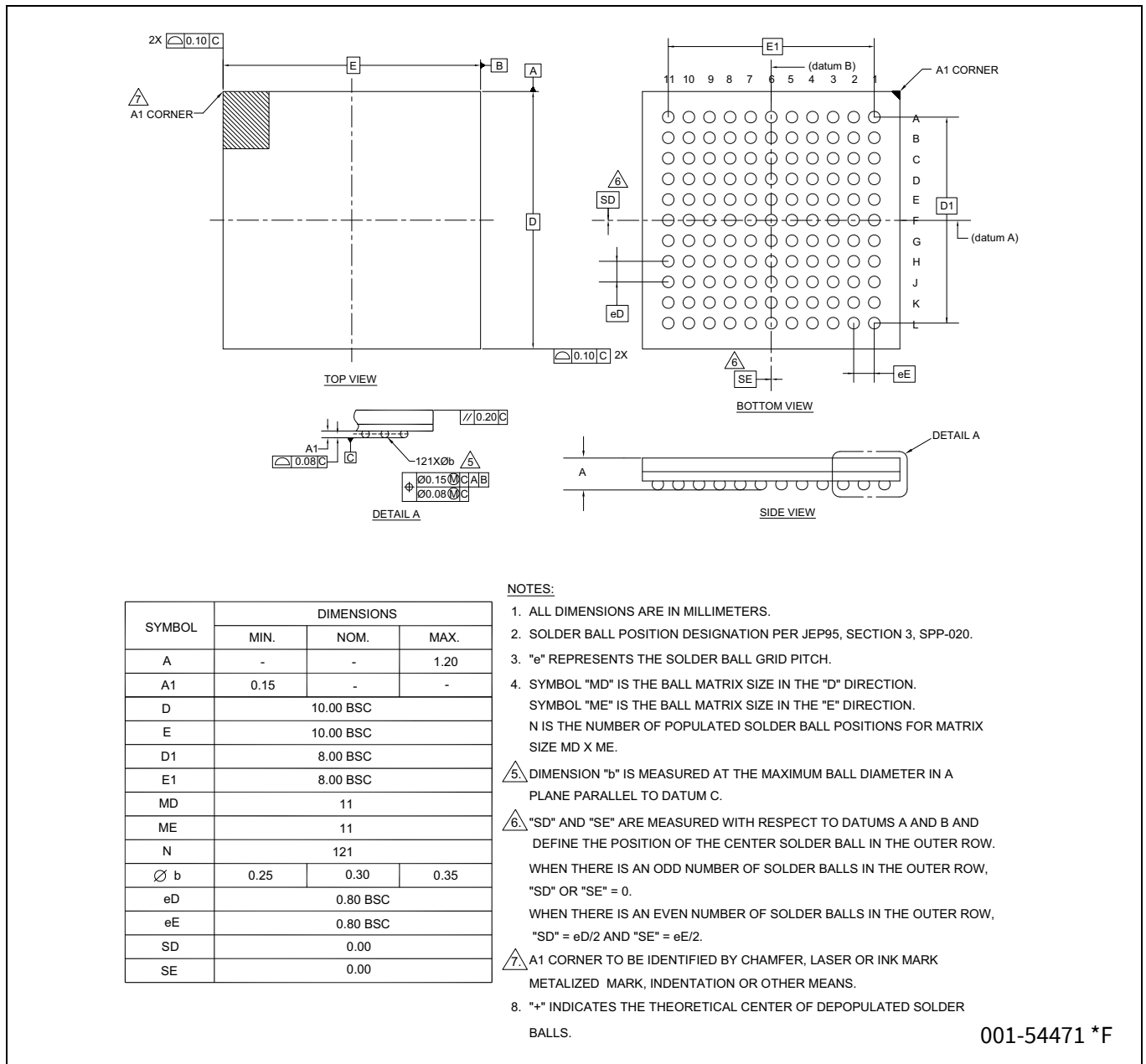
Figure 32 121-ball FBGA (10 × 10 × 1.2 mm (0.30 mm ball diameter)) package outline, 001-54471
