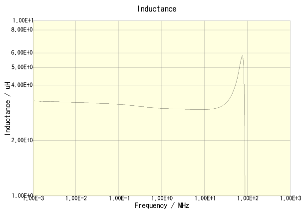
CLF7045T-3R3N-CA
