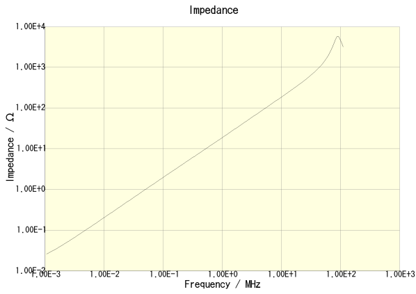
CLF7045T-3R3N-CA
