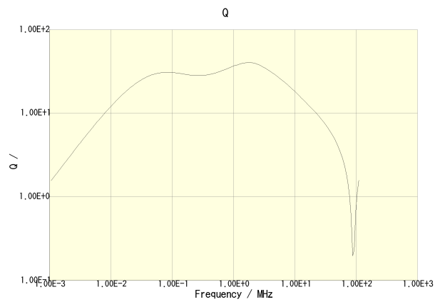
CLF7045T-3R3N-CA
