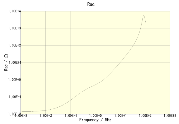
CLF7045T-3R3N-CA
