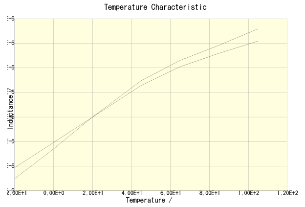
CLF7045T-3R3N-CA(DC = 0A)
