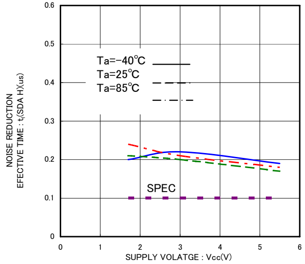
Fig.30 Noise reduction effective time t_1(\text{SDA H})
