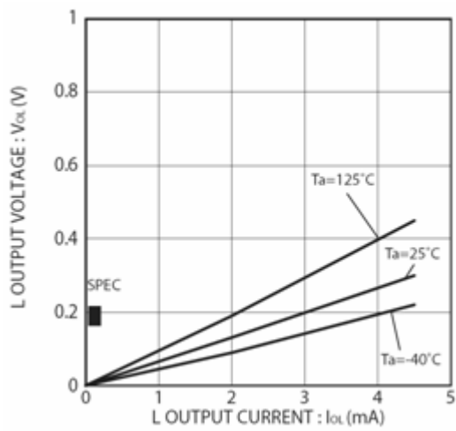
Figure 3. L output voltage VOL-IOL (VCC=2.7V)
