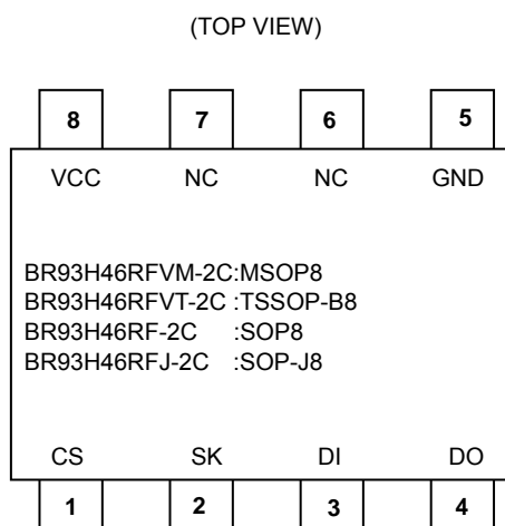
Figure 2. Pin Configuration
