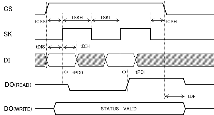
Figure 1. Serial Input / Output Timing Diagram
