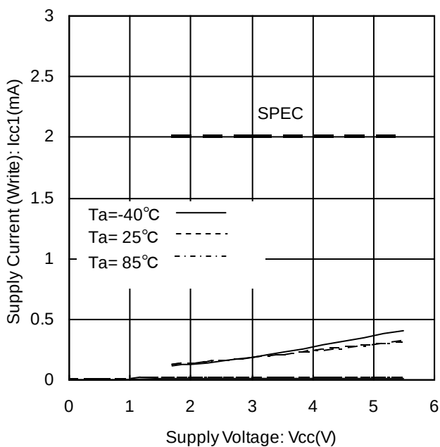
Figure 10. Supply Current (Write) vs Supply Voltage ( f_{SCL}=400\text{kHz} )
