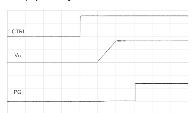
Start-up enabled by CTRL signal. \text{TON\_DELAY} = \text{TON\_RISE} = 10 \text{ ms} (default). V_i = 12 \text{ V} , I_o = \text{max } I_o , PG pulled up to V_o . Scale: 2 or 1 V/div, 10 ms/div. V_{out} = 1.8\text{V}
