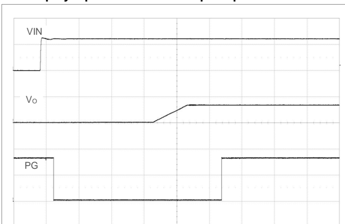
Start-up enabled by applying V_{in} . \text{TON\_DELAY} = \text{TON\_RISE} = 10 \text{ ms} (default). V_i = 12 \text{ V} , I_o = \text{max } I_o , PG pulled up to external 3.3V. Scale: 10 or 5 V/div, 10 ms/div. V_{out} = 3.3\text{V}
