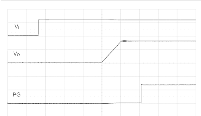
Start-up enabled by applying V_i . \text{TON\_DELAY} = \text{TON\_RISE} = 10 \text{ ms} (default). V_i = 12 \text{ V} , I_o = \text{max } I_o , PG pulled up to V_o . Scale: 10 or 1 V/div, 10 ms/div. V_{out} = 1.8\text{V}
