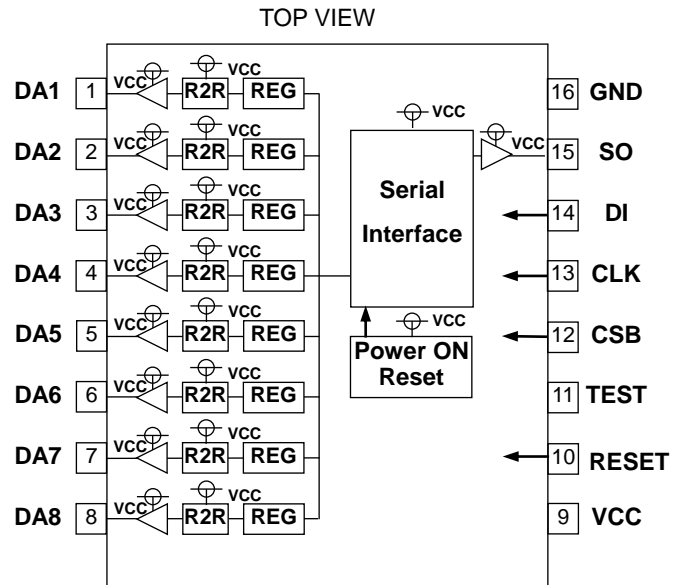
Figure 1. BH2226FV/BH2226F
