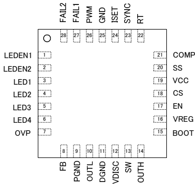
Fig.2 Pin configuration
