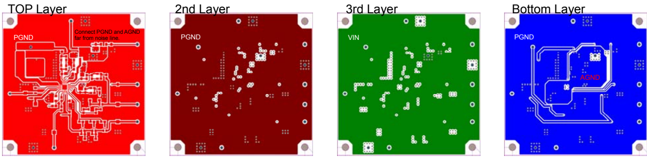
Figure 42. Recommended Layout Pattern
