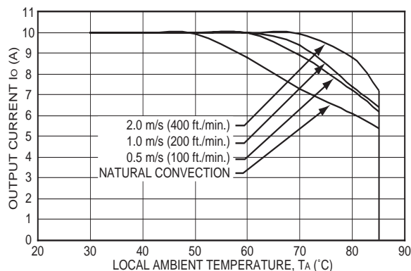
Figure 26. Typical Power Derating vs output Current for 3.3 Vin.
