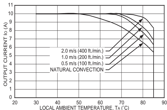
Figure 27. Typical Power Derating vs output Current for 5.0 Vin.
