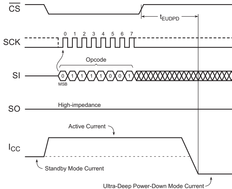
Figure 10-3. Ultra-Deep Power-Down
