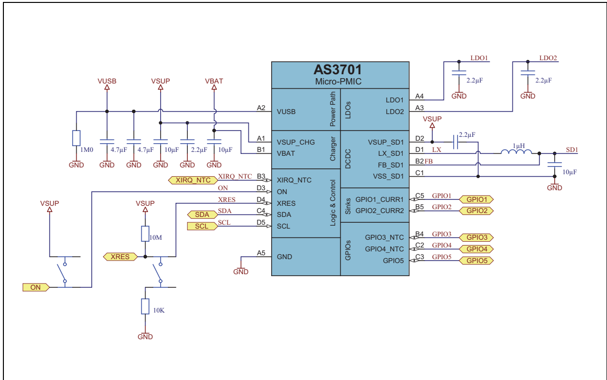
Figure 114: Application Schematic
