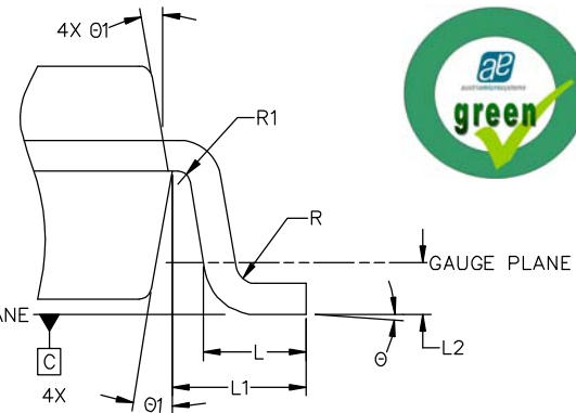
VIEW C
