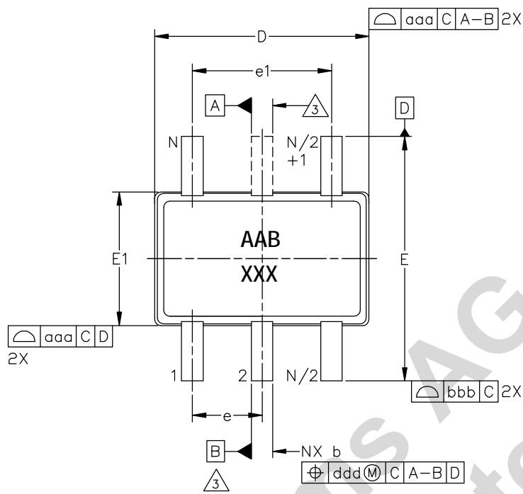
Figure 27. SC70-5 Package
