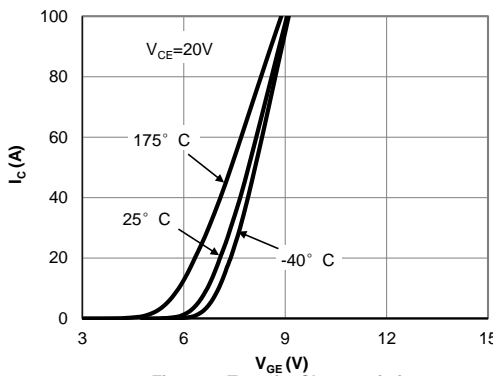
Figure 3: Transfer Characteristic
