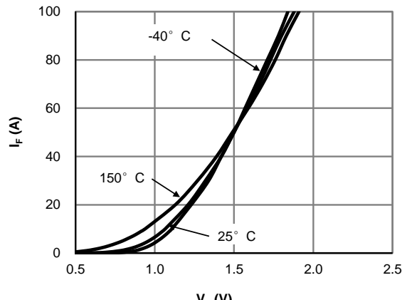
Fig 4: Diode Characteristic
