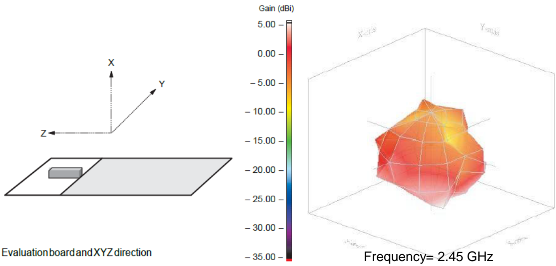
Radiation pattern
