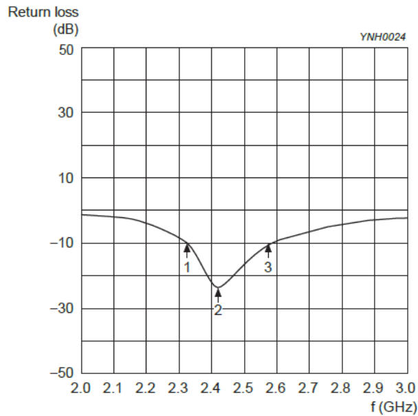
Return loss
