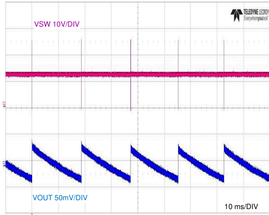
Figure 7-14. No-Load Switching
