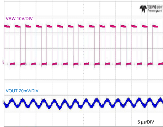
Figure 7-15. Full-Load Switching
