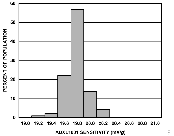
Figure 12. ADXL1001 Sensitivity Histogram at 25°C
