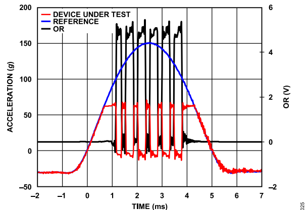
Figure 26. ADXL1001/ADXL1002 Behavior During a Continuous Overrange
