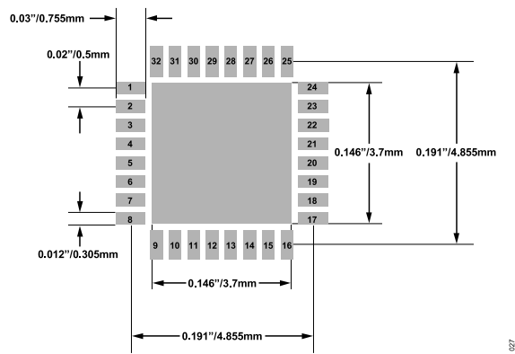
Figure 28. Recommended Printed Wiring Board Land Pattern
