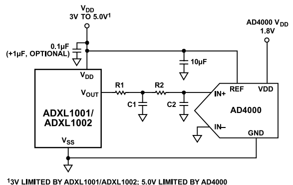
Figure 25. Application Circuit for the ADXL1001/ADXL1002
