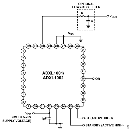
Figure 22. ADXL1001/ADXL1002 Application Circuit
