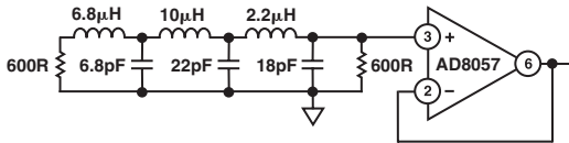
Figure 59. Example/Cr Output Filter: PS Mode/2x Oversampling
