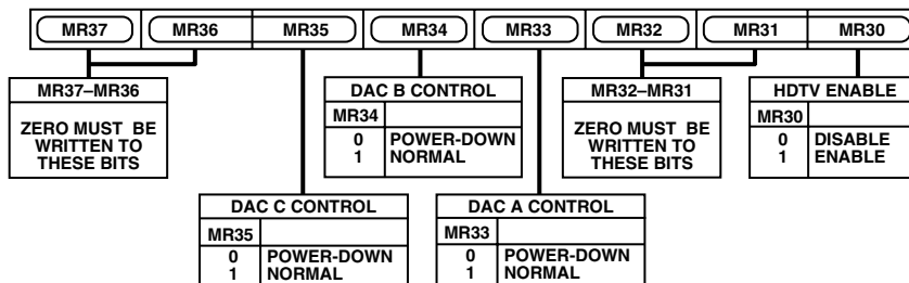
Figure 54. Mode Register 3
