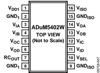
Figure 7. ADuM5402W Pin Configuration
