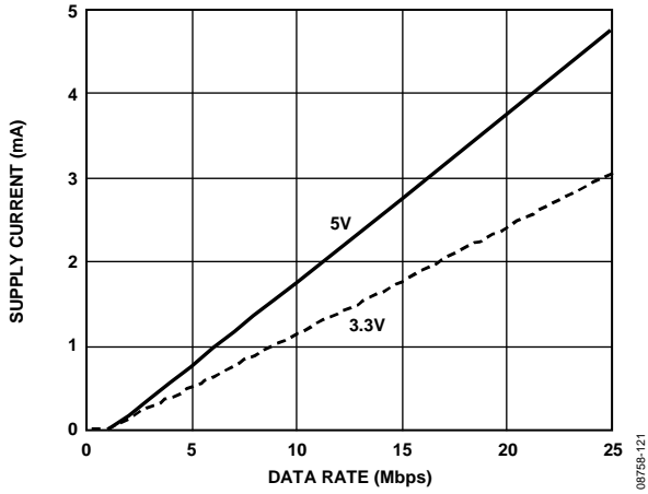
Figure 21. Typical I ISO(D) Dynamic Supply Current per Input
