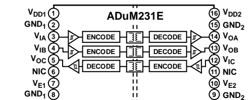
Figure 4. ADuM231E Functional Block Diagram
