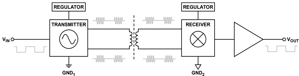
Figure 23. Operational Block Diagram of a Single Channel with a High Fail-Safe Output State
