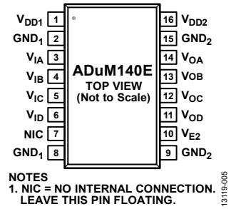
Figure 8. ADuM140E Pin Configuration
