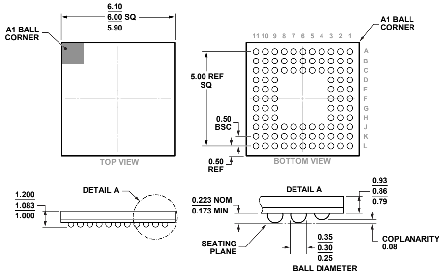
Figure 16. 96-Ball Chip Scale Package Ball Grid Array [CSP_BGA] (BC-96-2) Dimensions shown in millimeters
