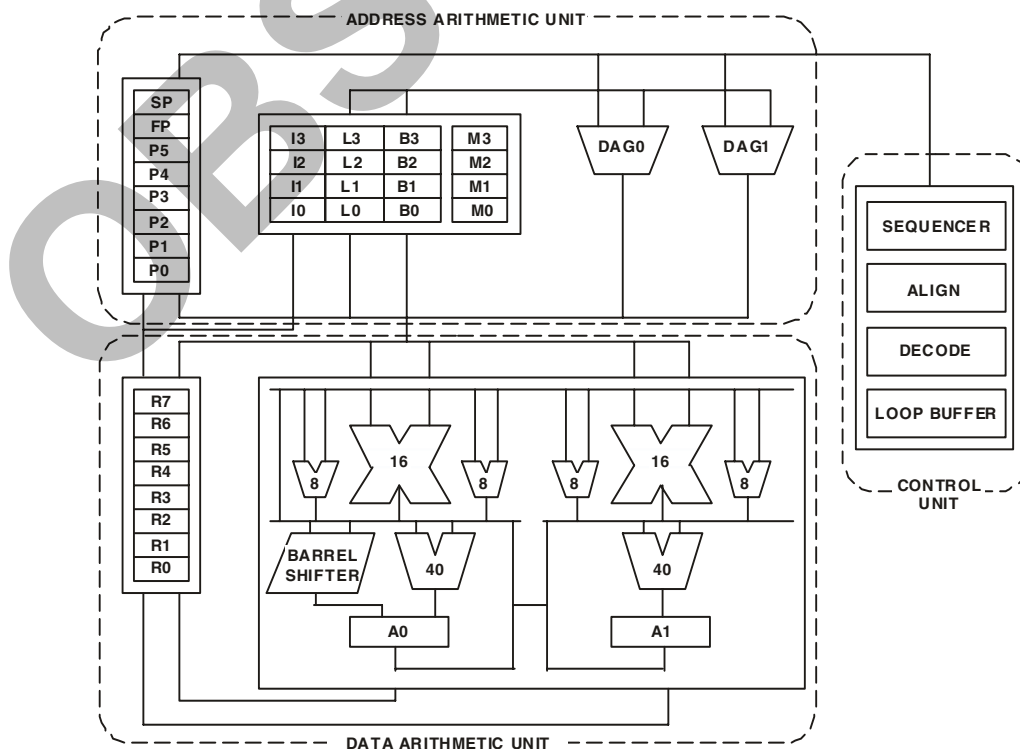
Figure 1. Processor Core
