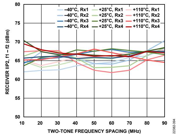
Figure 465. Receiver IIP2, f_1 - f_2 vs. Two-Tone Frequency Spacing, Both Tones at -11 dBFS, f_2 = 2 MHz
