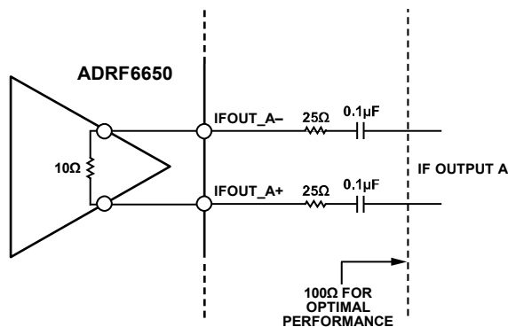
Figure 57. IF Output Schematic, Channel A Output Shown
