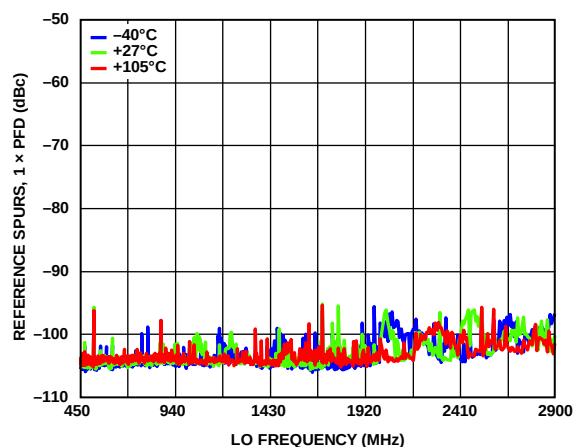
Figure 42. Reference Spurs vs. LO Frequency, 1 \times f_{PFD} Offset, Daisy-Chain Measurement
