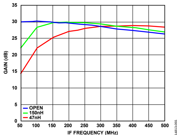
Figure 56. Centering the IF Bandwidth with L_{TUNEX} Gain vs. IF Frequency
