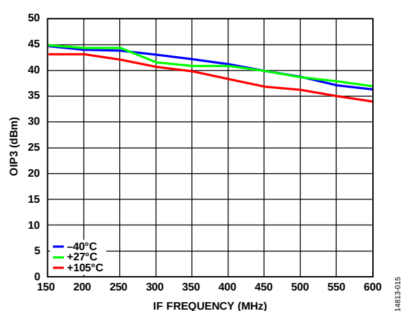
Figure 15. OIP3 vs. IF Frequency; RF Sweep with Fixed LO, Maximum Gain, L_{SHUNT} = 47 nH, IF = 368 MHz
