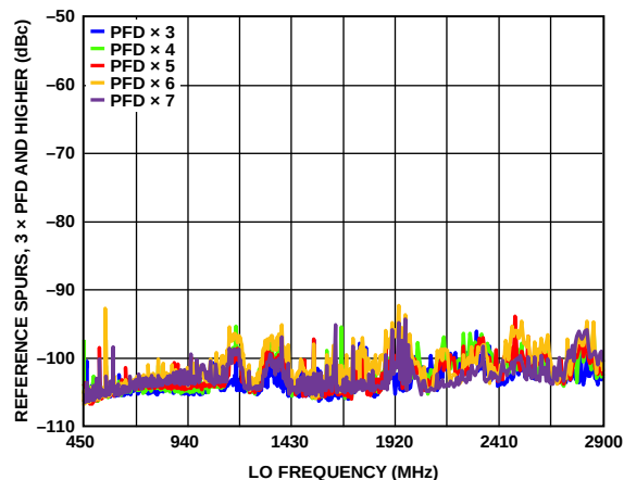
Figure 44. Reference Spurs vs. LO Frequency, 3 and Higher \times f_{PFD} Offset, Daisy-Chain Measurement
