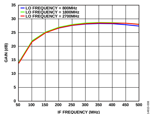
Figure 8. Gain vs. IF Frequency; RF Sweep with Fixed LO, L_{SHUNT} = 47\text{ nH}
