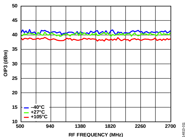
Figure 11. OIP3 vs. RF Frequency; Maximum Gain, L_{SHUNT} = 47 nH, IF = 368 MHz
