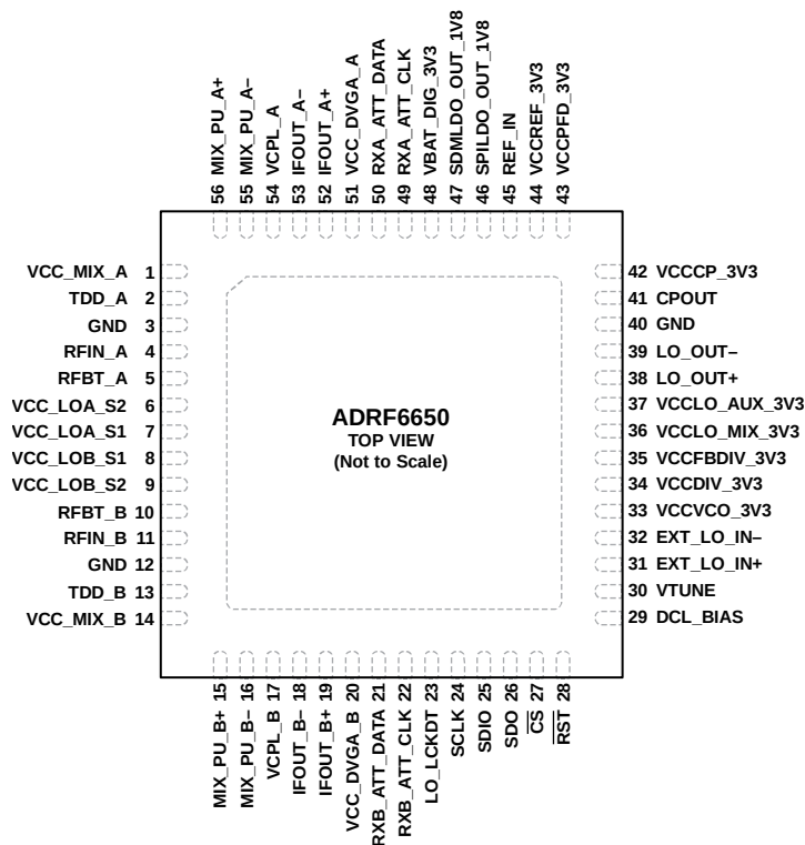
Figure 3. Pin Configuration
