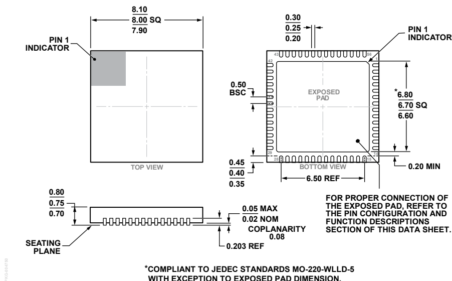
Figure 72. 56-Lead Lead Frame Chip Scale Package [LFCSP] 8 mm × 8 mm Body and 0.75 mm Package Height (CP-56-16)
