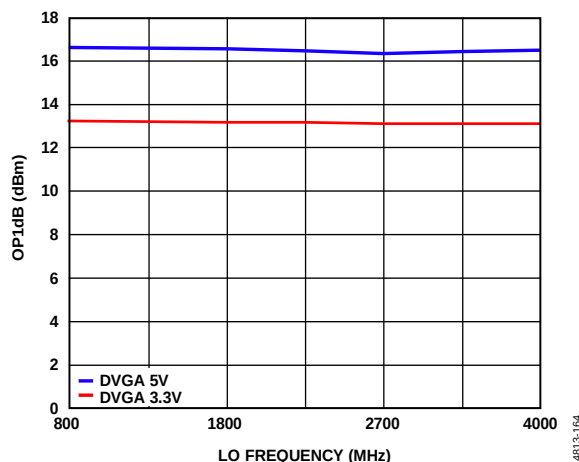
Figure 64. OP1dB vs. LO Frequency for Various Power Modes
