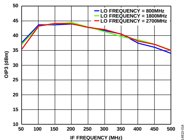
Figure 14. OIP3 vs. IF Frequency; RF Sweep with Fixed LO, Maximum Gain, L_{SHUNT} = 150 nH
