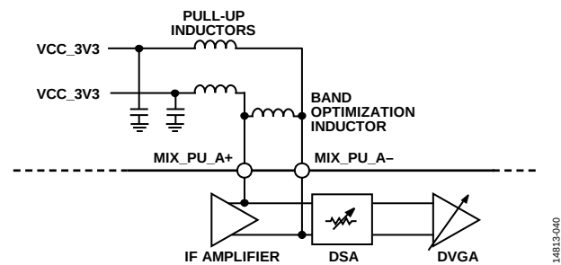
Figure 50. External Pull-Up Inductor Connection
