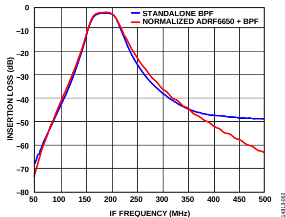
Figure 63. Standalone BPF and Normalized ADRF6650 and Band-Pass Filter Insertion Loss Response
