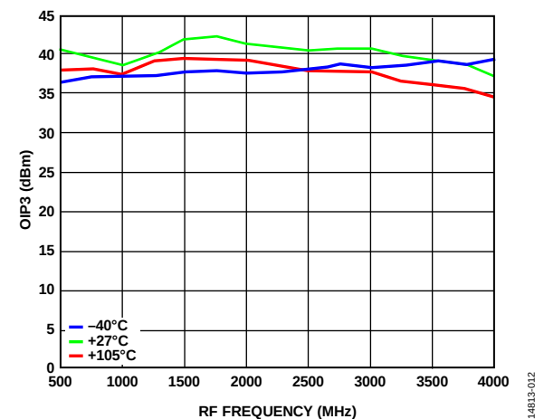
Figure 12. OIP3 vs. RF Frequency; Maximum Gain - 16 dB, L_{SHUNT} = 150 nH
