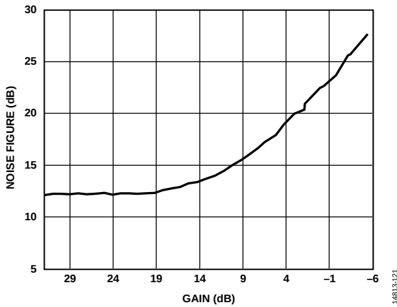
Figure 22. Noise Figure vs. Gain, RF = 2100 MHz
