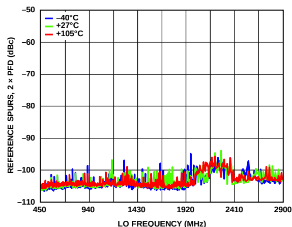
Figure 43. Reference Spurs vs. LO Frequency, 2 \times f_{PFD} Offset, Daisy-Chain Measurement
