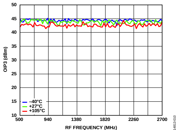
Figure 10. OIP3 vs. RF Frequency; Maximum Gain, L_{SHUNT} = 150 nH
