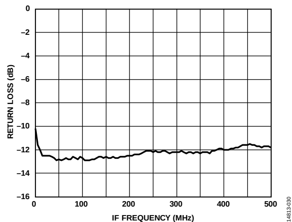
Figure 31. IF Output Return Loss, External 25 \Omega on Each Differential Leg
