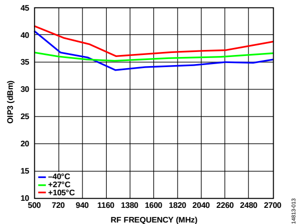
Figure 13. OIP3 vs. RF Frequency; Maximum Gain - 16 dB, L_{SHUNT} = 47 nH, IF = 368 MHz
