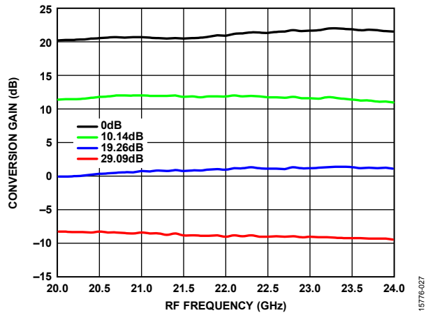
Figure 27. Conversion Gain vs. RF Frequency at Various Attenuation Levels, Upper Sideband
