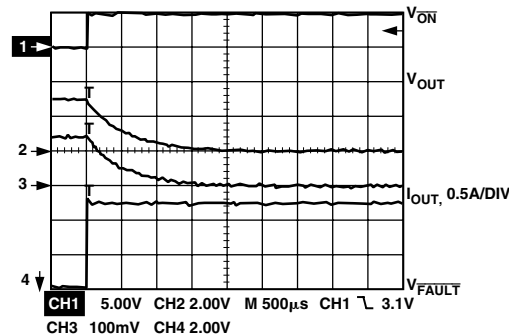
TPC 16. USB Circuit Output Fall Time
