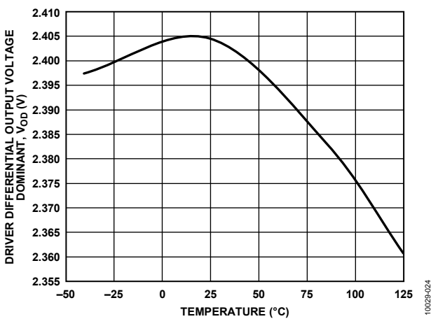
Figure 17. Driver Differential Output Voltage Dominant vs. Temperature
