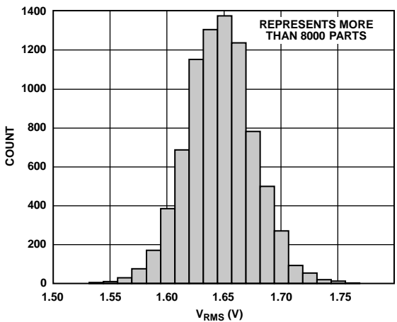
Figure 29. Distribution of V_{RMS} , P_{IN} = 8 \text{ dBm} , 900 MHz
