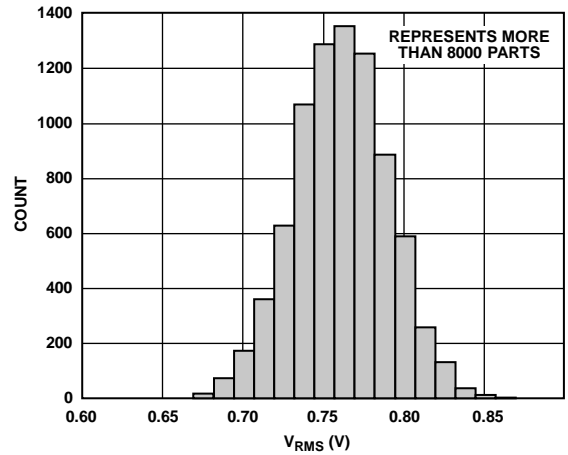
Figure 32. Distribution of V_{RMS} , P_{IN} = -16 \text{ dBm} , 900 MHz
