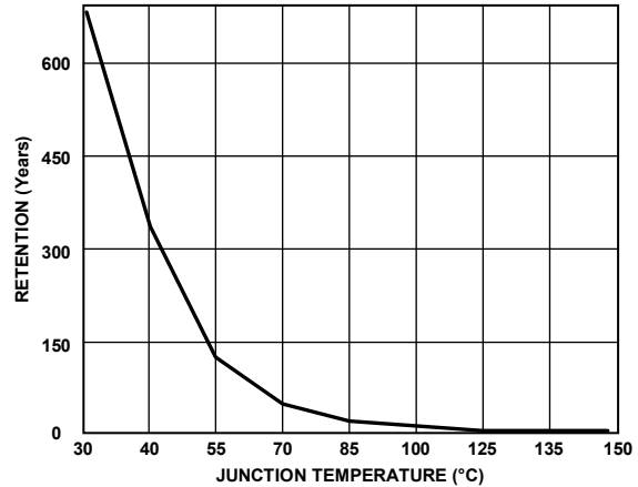
Figure 60. Flash Memory Retention
