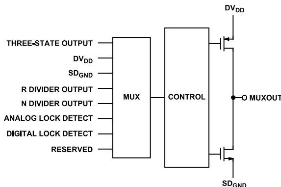
Figure 32. MUXOUT Schematic
