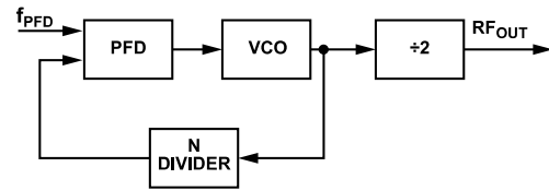
Figure 52. Loop Closed Before Output Divider
