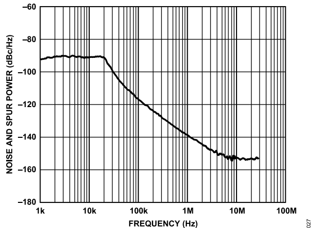
Figure 27. Fractional-N Spur Performance, RF_{OUTA+} = 2.591 GHz, f_{REFIN} = 122.88 MHz, f_{PFD} = 61.44 MHz, Output Divide by 2 Selected, Loop Filter Bandwidth = 10 kHz, Channel Spacing = 20 kHz
