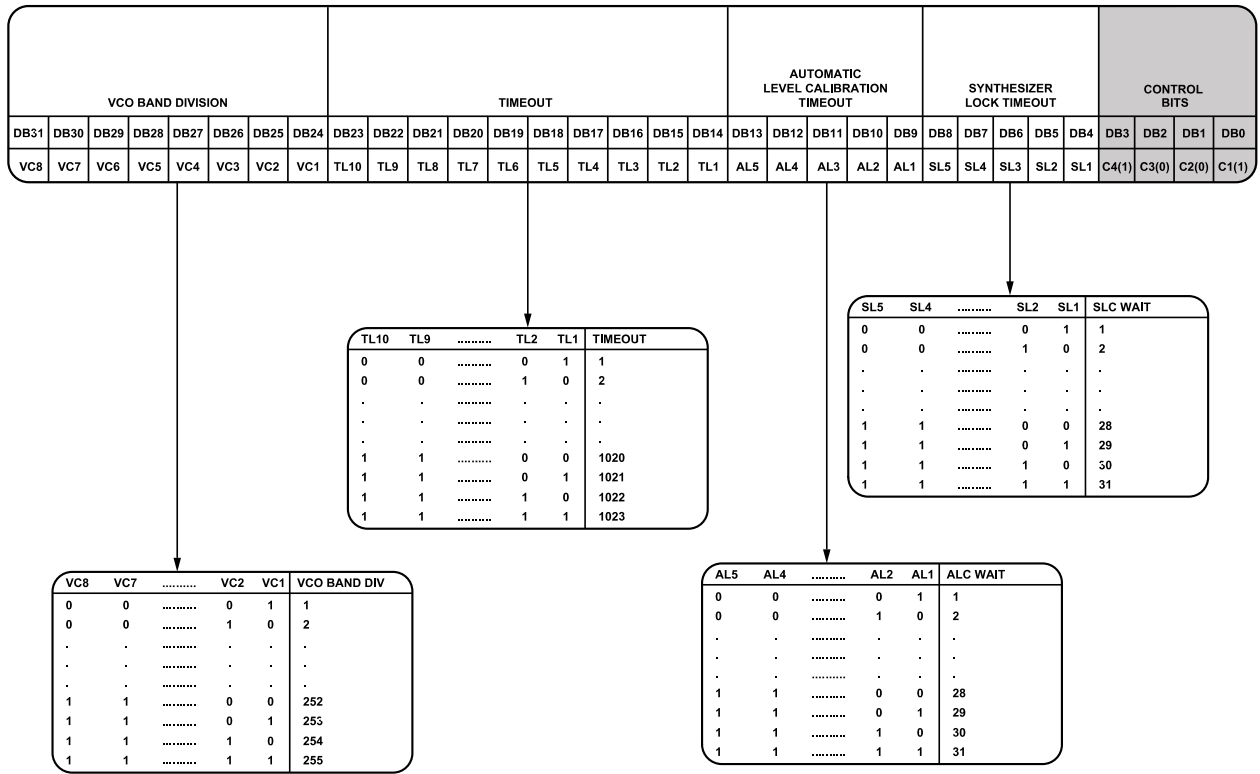
Figure 47. Register 9 Details
