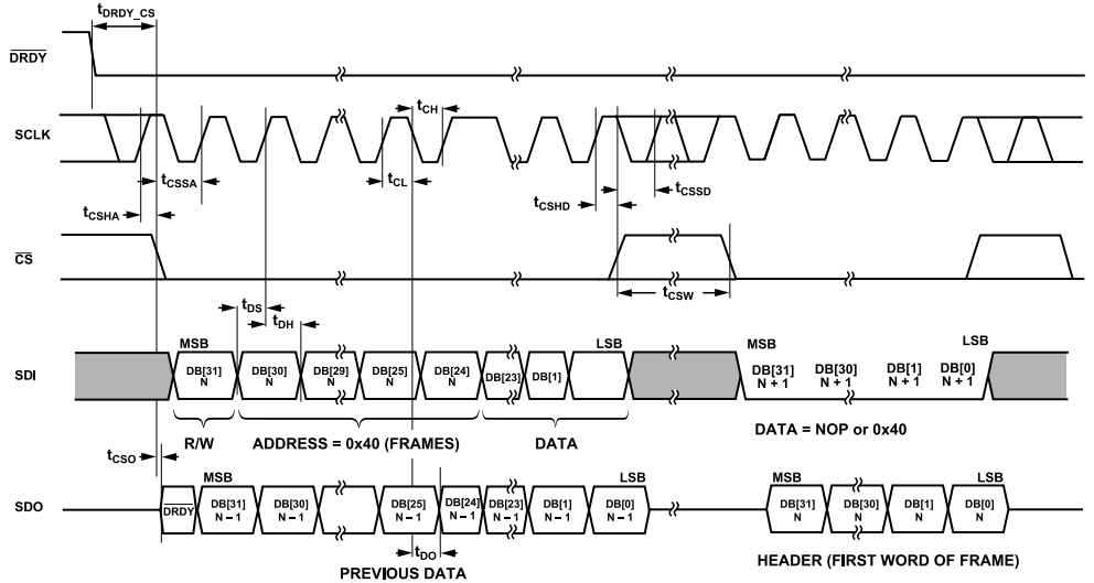
Figure 3. Starting Read Frame Data (CPHA = 1, CPOL = 1)
