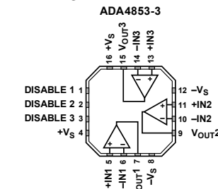
Figure 3. 16-Lead LFCSP_WQ
