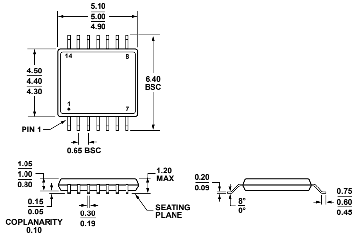
COMPLIANT TO JEDEC STANDARDS MO-153-AB-1 Figure 86. 14-Lead Thin Shrink Small Outline Package [TSSOP] (RU-14) Dimensions shown in millimeters
