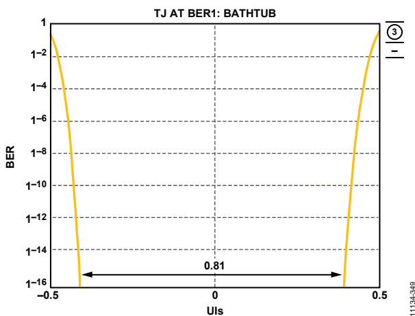
Figure 51. Digital Outputs Bathtub, External 100 \Omega Terminations at 2.5 Gbps
